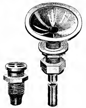
Fig. 3474. DRIP COUPLINGS.
